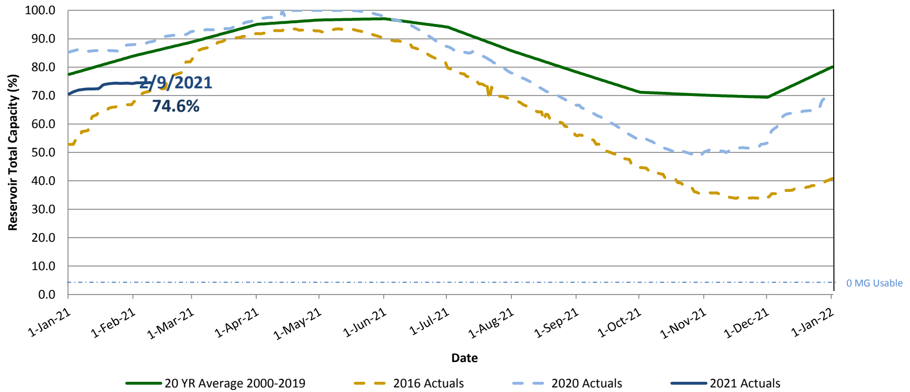
2021 Stamford System Reservoir Status (Usable Storage: 4,692 MG)
